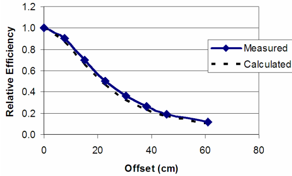
Figure 5 Change of Efficiency with Offset at Standoff of 20 cm.
