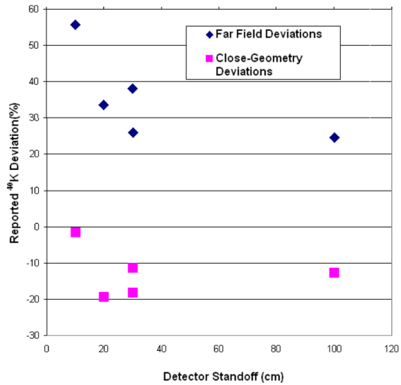
Figure 6 Comparison of Close-in Geometry and Far-Field Algorithms for the KCl Box.
