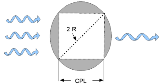
Figure 2 Top View of a Detector to Estimate the Average Penetration Distance.
