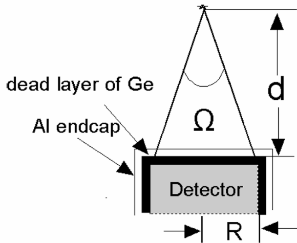
Figure 1 HPGe Detector with a Germanium Dead Layer and an Aluminum Endcap.
