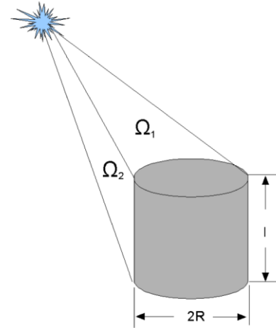
Figure 3 Activity of a Point Source Interacting with the Top and Side Surfaces of a Detector.
